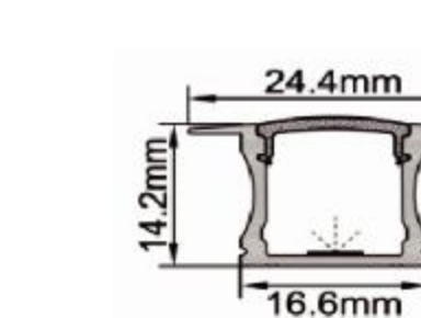
IC-061W-AP1714 PC Ice white diffuser mask "A" Alu+Silky silver finish Thickness of PC: 0.85mm Thickness of Alu: 0.85mm
