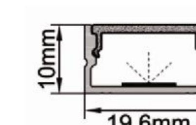
IC-012-AP2010 PC Ice white diffuser mask "A" Alu+Silky silver finish Thickness of PC: 0.85mm Thickness of Alu: 0.80mm
