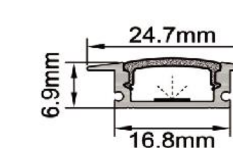
IC-070W-AP1707 PC Ice white diffuser mask "A" Alu+Silky silver finish Thickness of PC: 0.85mm Thickness of Alu: 0.70mm
