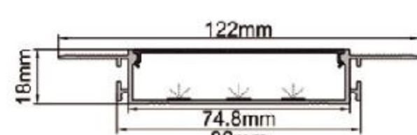
IC-371UP-PE7518 PC Ice white diffuser mask "A" Alu+Silky silver finish Thickness of PC: 1.30mm Thickness of Alu: 1.20mm
