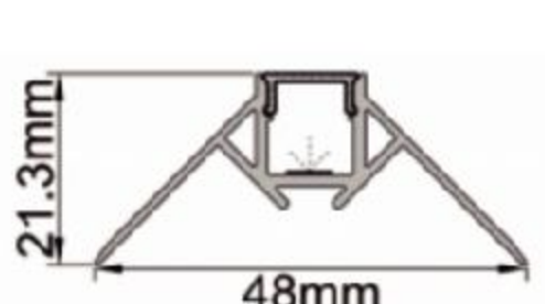
IC-338N-PE4821 PC Ice white diffuser mask "A" Alu+Silky silver finish Thickness of PC: 0.75mm Thickness of Alu: 1.20mm
