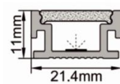
IC-212-UL2111 PC Ice white diffuser mask "A" Alu+Silky silver finish Thickness of PC: 2.60mm Thickness of Alu: 1.15mm
