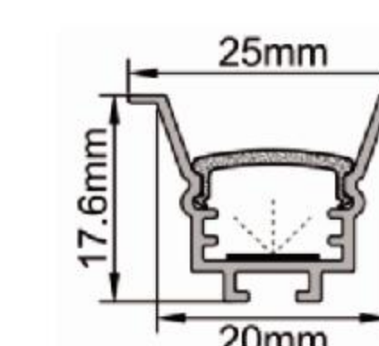
IC-177-AP2018 PC Ice white diffuser mask "A" Alu+Silky silver finish Thickness of PC: 0.85mm Thickness of Alu: 0.70mm
