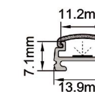
IC-077-AP1307 PC Ice white diffuser mask "A" Alu+Silky silver finish Thickness of PC: 0.80mm Thickness of Alu: 0.70mm
