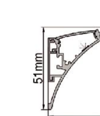
IC-354-AP5136 PC Ice white diffuser mask "A" Alu+Silky silver finish Thickness of PC: 0.90mm Thickness of Alu: 0.95mm
