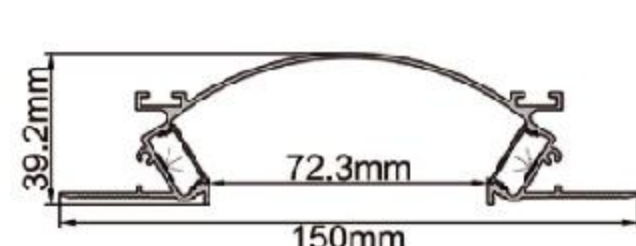
IC-328-PE15040 PC Ice white diffuser mask "A" Alu+Silky silver finish Thickness of PC: 0.90mm Thickness of Alu: 1.20mm
