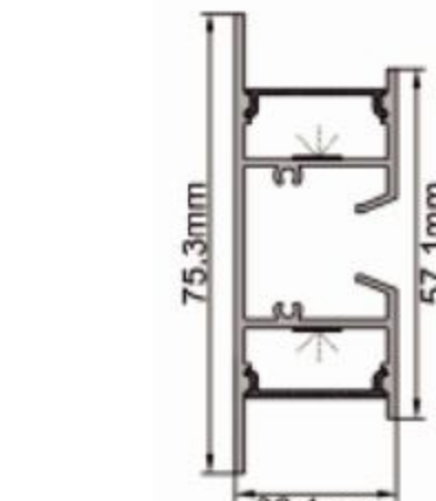
IC-150-AP7526 PC Ice white diffuser mask "A" Alu+Silky silver finish Thickness of PC: 1.00mm Thickness of Alu: 1.30mm
