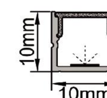
IC-083-AP1010 PC Ice white diffuser mask "A" Alu+Silky silver finish Thickness of PC: 0.80mm Thickness of Alu: 0.70mm
