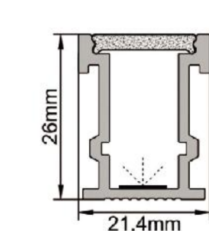
IC-231-UL2126 PC Ice white diffuser mask "A" Alu+Silky silver finish Thickness of PC: 2.60mm Thickness of Alu: 1.25mm
