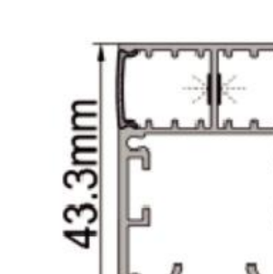
IC-151-AP2843 PC Ice white diffuser mask "A" Alu+Silky silver finish Thickness of PC: 0.80mm Thickness of Alu: 1.05mm
