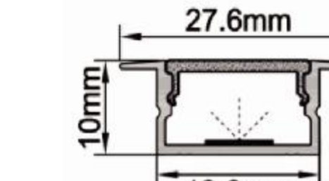
IC-012W-AP2010 PC Ice white diffuser mask "A" Alu+Silky silver finish Thickness of PC: 0.85mm Thickness of Alu: 0.80mm
