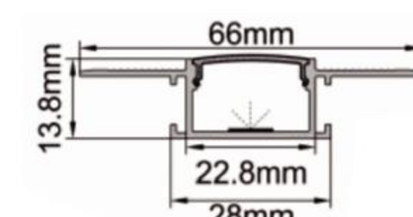
IC-303UP-PE2313 PC Ice white diffuser mask "A" Alu+Silky silver finish Thickness of PC: 0.85mm Thickness of Alu: 0.95mm
