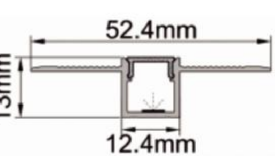
IC-330UP-PE1313 PC Ice white diffuser mask "A" Alu+Silky silver finish Thickness of PC: 0.75mm Thickness of Alu: 0.95mm
