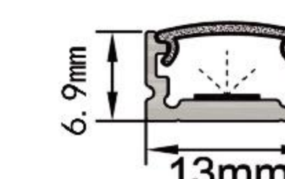
IC-055-AP1307 PC Ice white diffuser mask "A" Alu+Silky silver finish Thickness of PC: 0.80mm Thickness of Alu: 1.25mm
