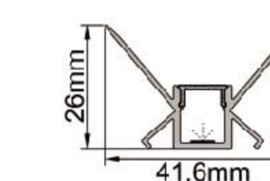
IC-338V-PE4226 PC Ice white diffuser mask "A" Alu+Silky silver finish Thickness of PC: 0.75mm Thickness of Alu: 1.20mm
