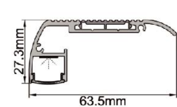
IC-733-SS6327 PC Ice white diffuser mask "A" Alu+Silky silver finish Thickness of PC: 0.75mm Thickness of Alu: 2.50mm
