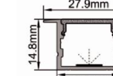
IC-065W-AP2015 PC Ice white diffuser mask "A" Alu+Silky silver finish Thickness of PC: 0.85mm Thickness of Alu: 0.75mm
