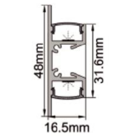
IC-712-AP4816 PC Ice white diffuser mask "A" Alu+Silky silver finish Thickness of PC: 0.90mm Thickness of Alu: 1.30mm
