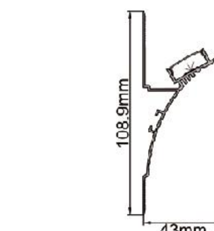
IC-363UP-PE10843 PC Ice white diffuser mask "A" Alu+Silky silver finish Thickness of PC: 0.90mm Thickness of Alu: 1.30mm
