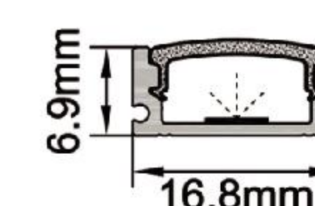
IC-070-AP1707 PC Ice white diffuser mask "A" Alu+Silky silver finish Thickness of PC: 0.85mm Thickness of Alu: 0.70mm
