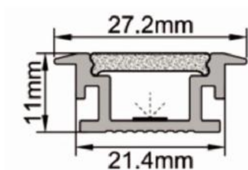
IC-212W-UL2111 PC Ice white diffuser mask "A" Alu+Silky silver finish Thickness of PC: 2.60mm Thickness of Alu: 1.15mm
