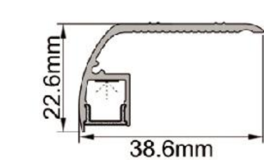
IC-729-SS3922 PC Ice white diffuser mask "A" Alu+Silky silver finish Thickness of PC: 0.80mm Thickness of Alu: 1.80mm
