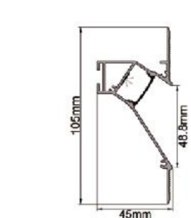
IC-64-PE10545 PC Ice white diffuser mask "A" Alu+Silky silver finish Thickness of PC: 0.90mm Thickness of Alu: 1.20mm
