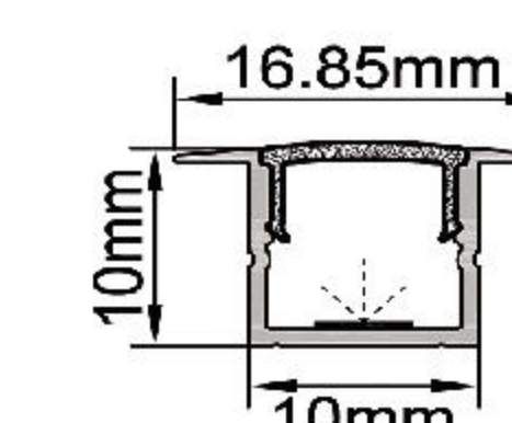
IC-083W-AP1010 PC Ice white diffuser mask "A" Alu+Silky silver finish Thickness of PC: 0.80mm Thickness of Alu: 0.70mm
