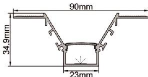
IC-315UP-PE9035 PC Ice white diffuser mask "A" Alu+Silky silver finish Thickness of PC: 0.90mm Thickness of Alu: 1.20mm
