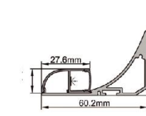
IC-047-AP6037 PC Ice white diffuser mask "A" Alu+Silky silver finish Thickness of PC: 0.80mm Thickness of Alu: 1.30mm
